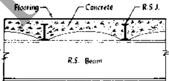
Fig 12.8 (b) Concrete jack floor
