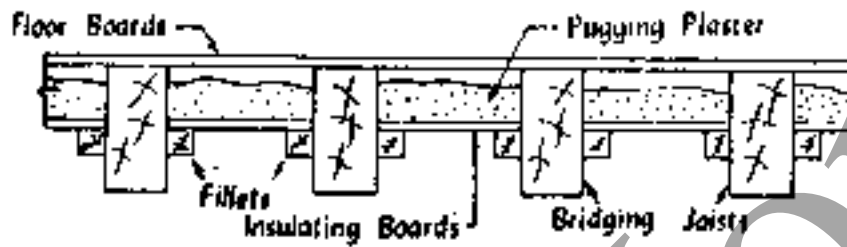
Fig 12.1 Pugging
