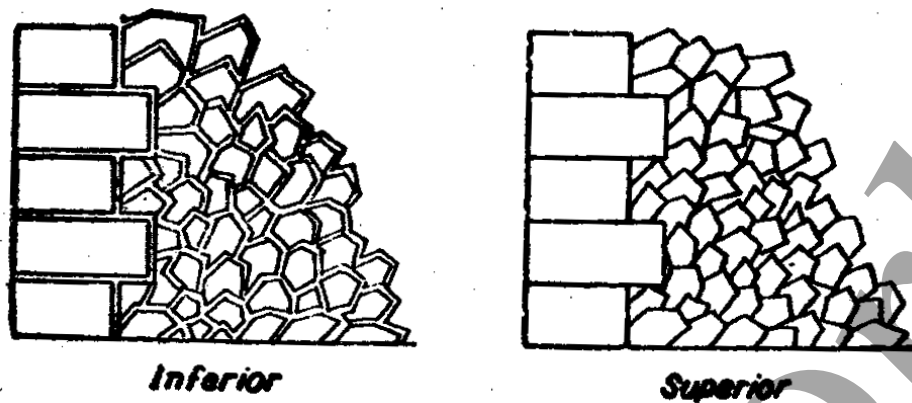
Fig. 11.8 Polygonal rubble masonry
