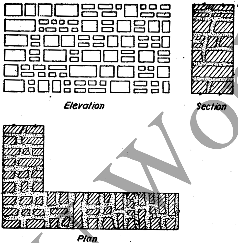
Fig 11.6 Coursed Squared Rubble Masonry
