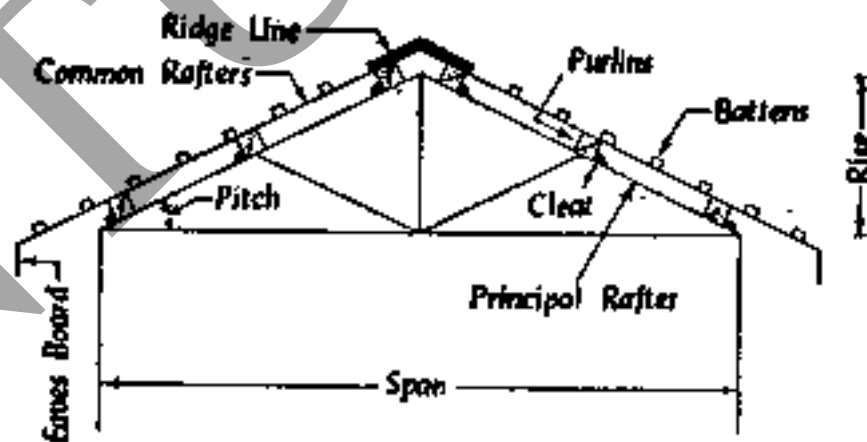
Fig 13.2 Truss
