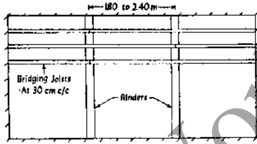
Plan of double joist timber floor
