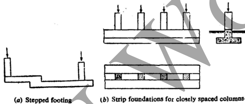
Fig 10.7 Continuous Footing
