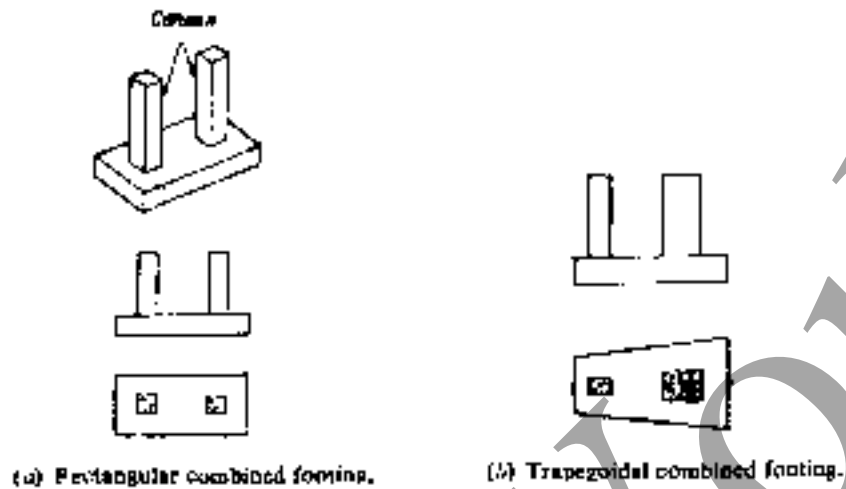
Fig 10.5 Combined Footings
