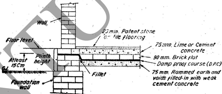
Fig 14.1 D.P.C. above ground level for new buildings
