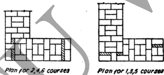
Two-bricks double flemish bond.
