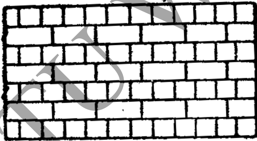
Fig 11.22 Dutch Bond
