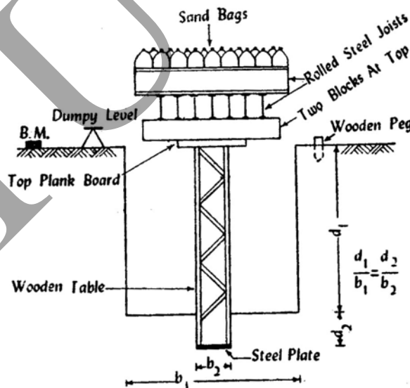
Fig 10.1 Method of loading
