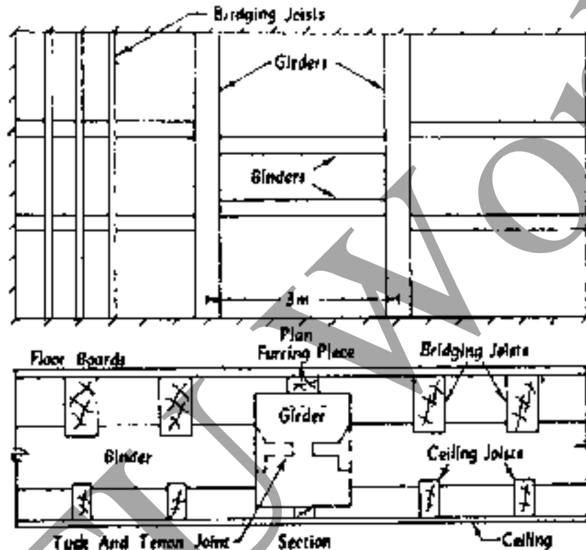
Fig 12.5 Details of framed timber floors
