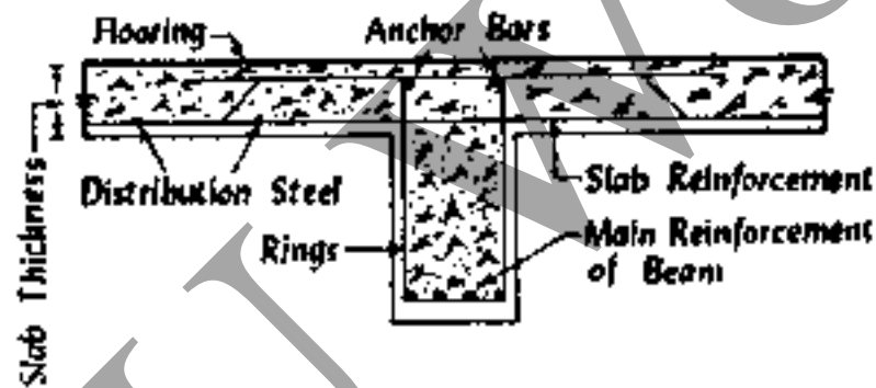
Fig 12.9 R.C.C. Floor
