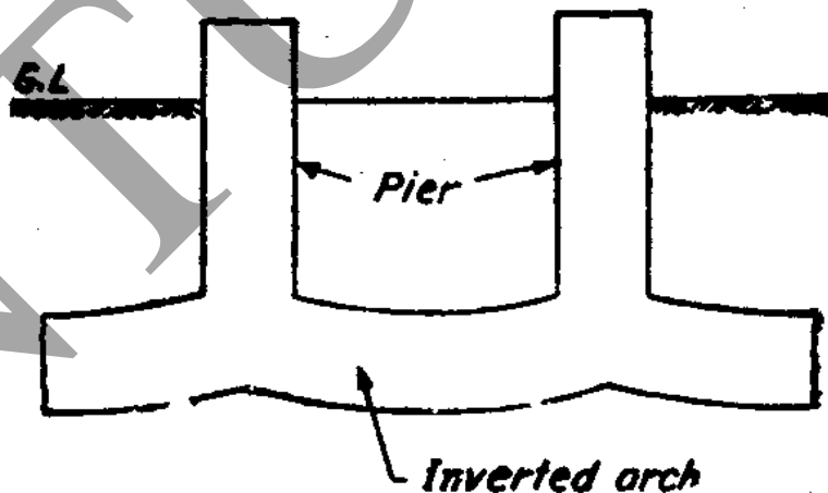
Fig 10.6 Inverted Footing
