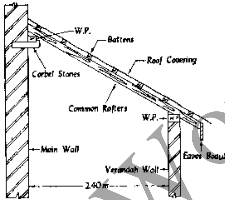
Fig 13.3 Lean-to roof
