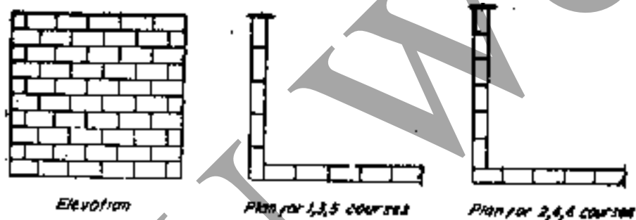
Fig 11.14 Stretcher Bond
