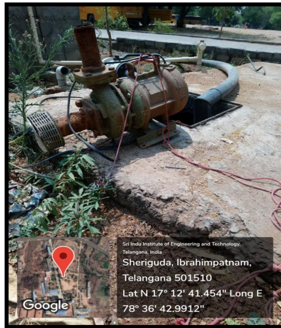
Treated Waste water stores in tank and supplies through motor pump system
