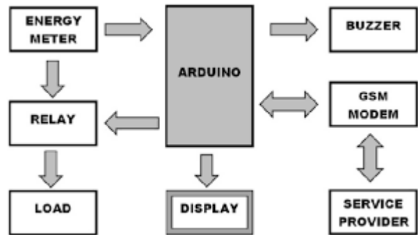
Fig:3 Block diagram
