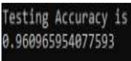
Fig. Accuracy
