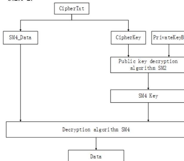
Figure 3.2.1-2: Decryption flowchart
