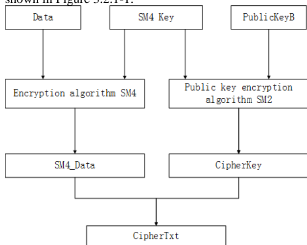
Figure 3.2.1-1: Encryption flowchart
