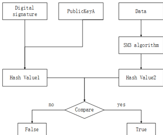
Figure 3.2.1-2: Verification flowchart
