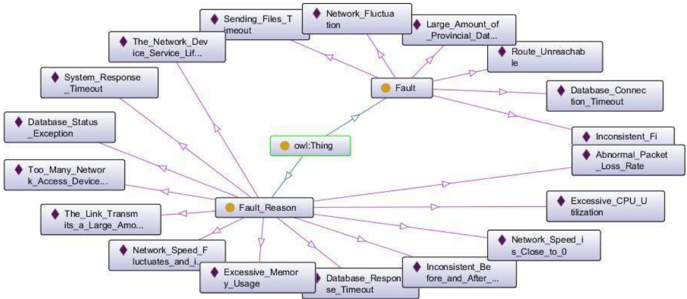
Figure 2: Ontology hierarchy
