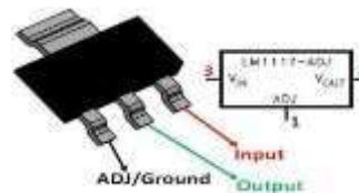
Fig 2.voltage regulator (LM1117)
