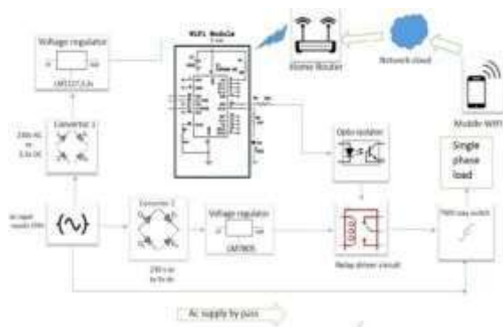
Fig.1.Functional Diagram of Smart Switch
