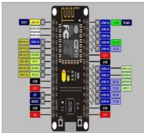
Figure 4 : Node MCU
