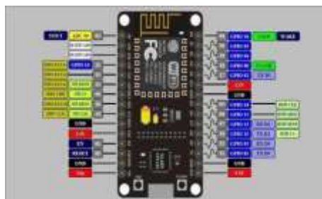
Fig 1: Node MCU
