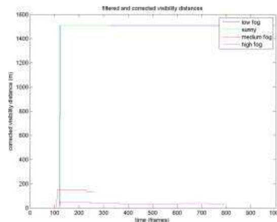
(b) Corrected visibility distance taking in consideration Sobel edge information
