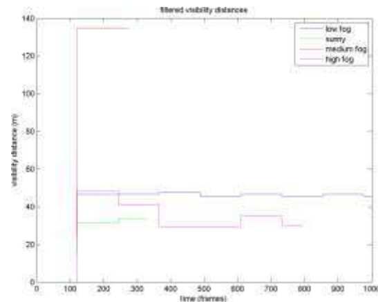
(a) Corrected visibility distance without taking in consideration Sobel edge information
