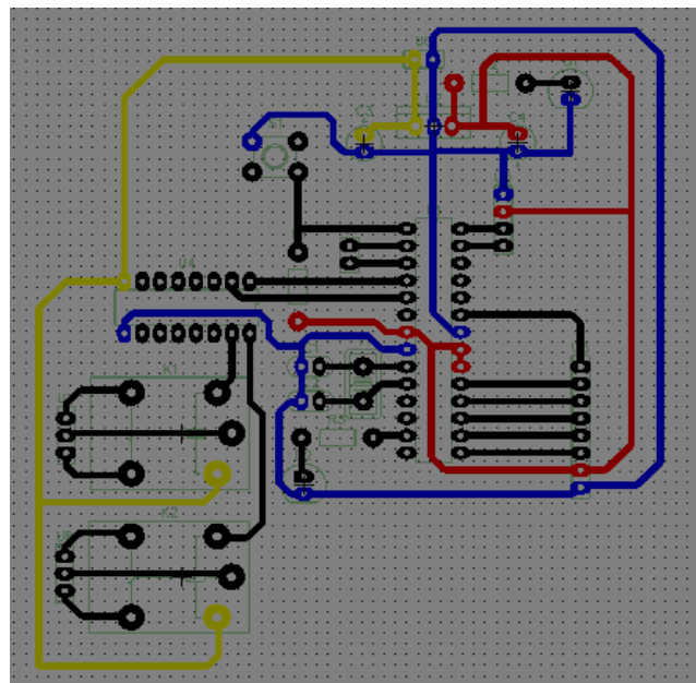
Fig 3- Circuit designing by DipTrace software
